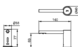
TLK01101AA Touchless Soap Dispenser(Controller) 3 Ltr – 1Way
