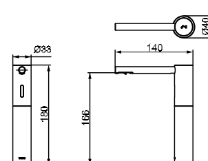
TLK01101AA Touchless Soap Dispenser(Controller) 3 Ltr – 1Way
