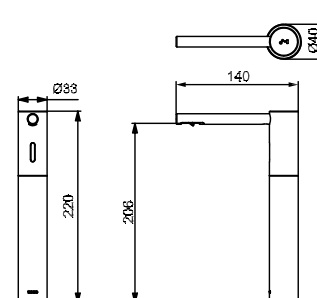
TLK01101AA Touchless Soap Dispenser(Controller) 3 Ltr – 1Way
